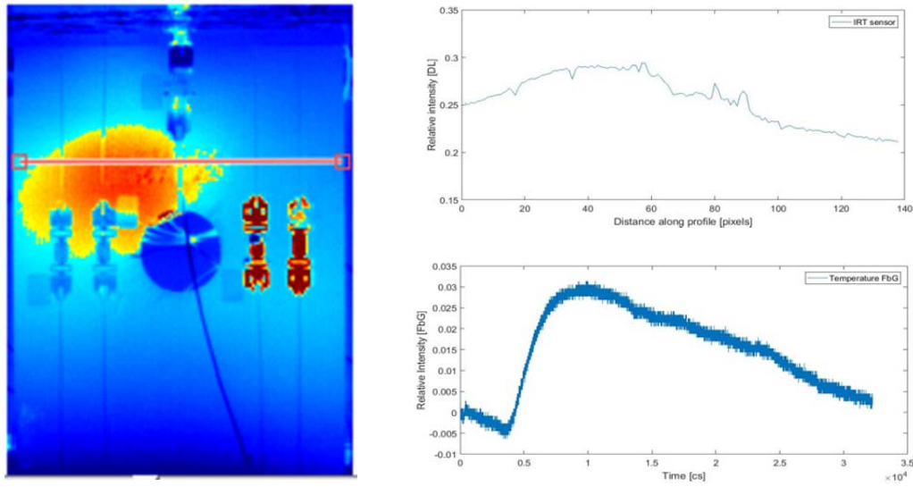
Fig. 3. Results obtained by IRT (left and top right) and FBG (bottom right) sensors in the tests for localized heating areas.
