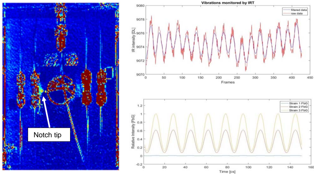
Fig. 4. Results obtained by IRT (left and top right) and FBG (bottom right) sensors in the low energy vibration tests.
