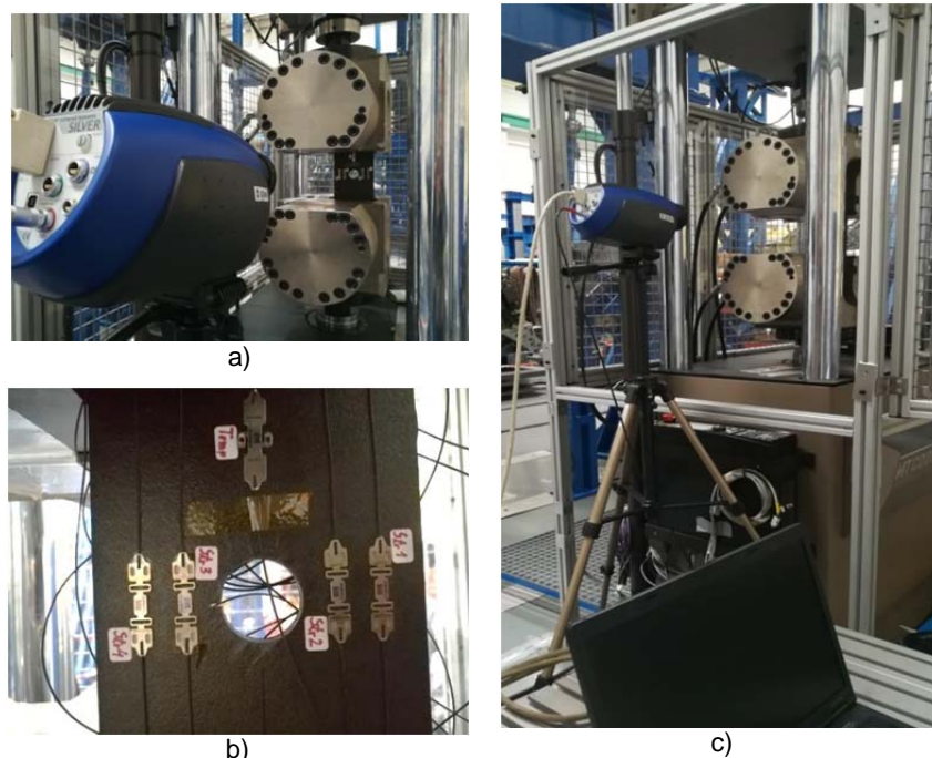
Fig. 2. Images of the preliminary test campaign. (a,c) Detail and general IRT monitoring setup, (b) positions of FBG sensors in a CFRP sample.
