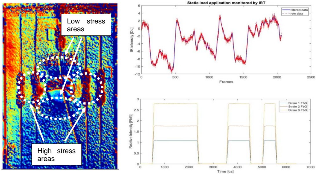
Fig. 5. Results obtained by IRT (left and top right) and FBG (bottom right) sensors in the static load tests.
