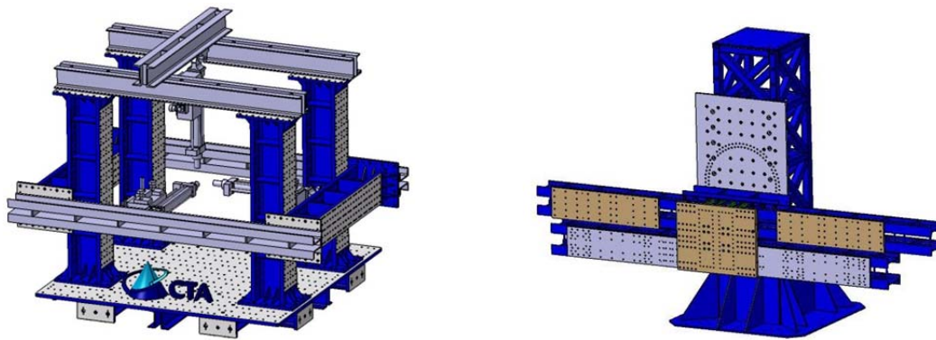
Fig. 1. Examples of conventional tooling made of rigid steel profiles assembled by screws.
