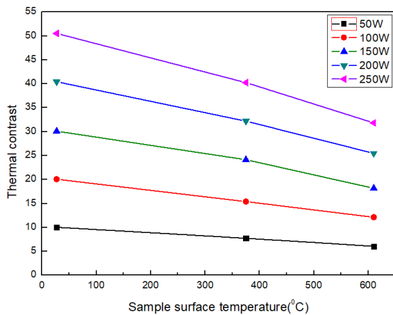
Fig.3 Influence of scanning laser power on thermal contrast
